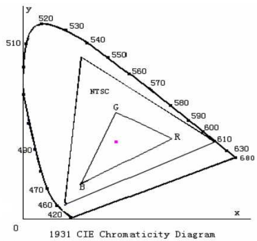
Fig.4. 1931 CIE chromaticity diagram
